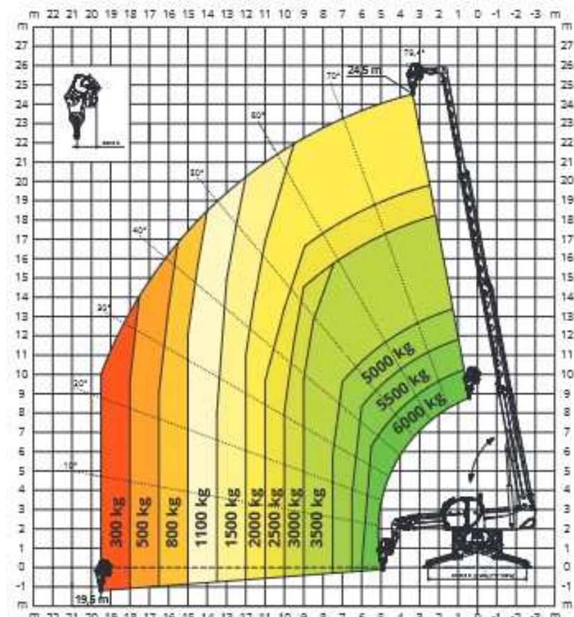
Teleskopstapler Roto TR 60-25 / 6t Winde (Magni RTH 6.25SH)
