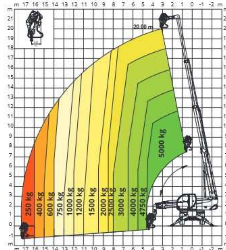
Teleskopstapler Roto R 50-21 / 5,0t Winde (Magni RTH 5.21)
