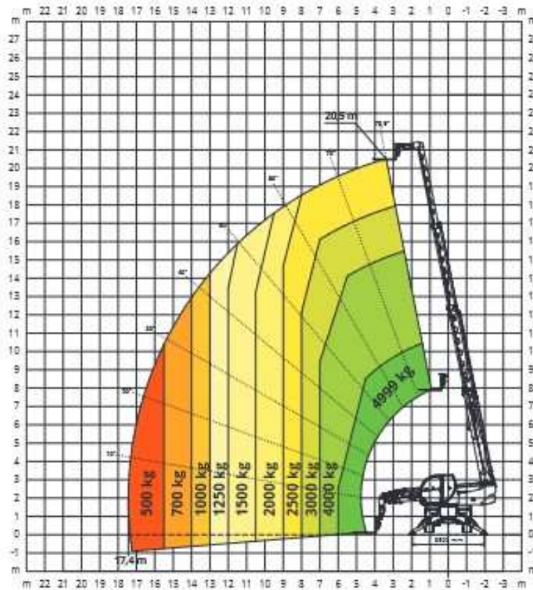
Teleskopstapler Roto R 50-21 / 1,2m Lastgabel (Magni RTH 5.21)
