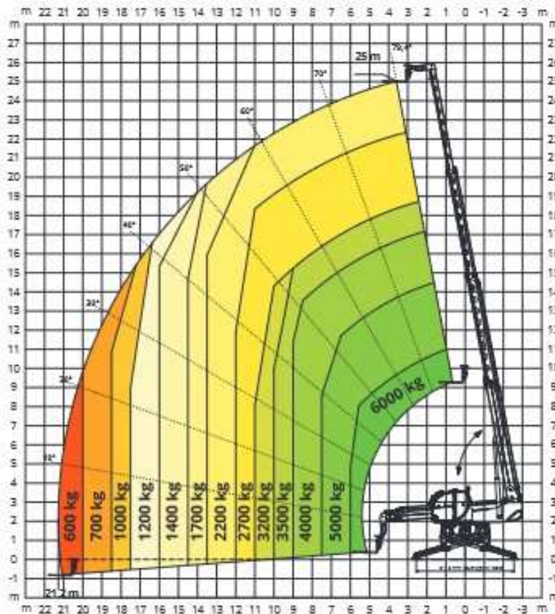
Teleskopstapler Roto TR 60-25 / 1,2m Lastgabel (Magni RTH 6.25SH)
